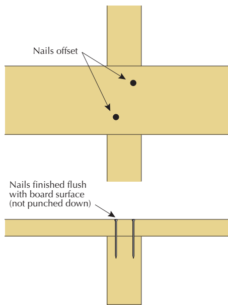
Figure 5: Nailing at intermediate locations
