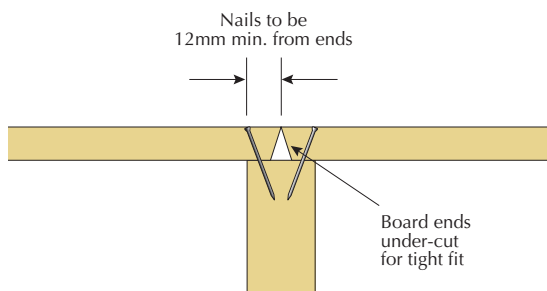
Figure 6: Nailing at board ends
