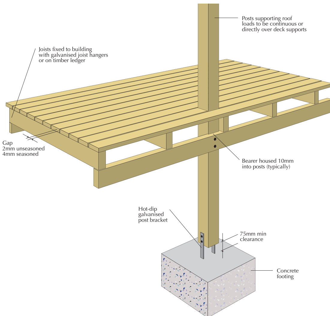
Figure 1: Typical domestic deck construction
