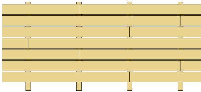
Figure 4: Staggered deck board ends
