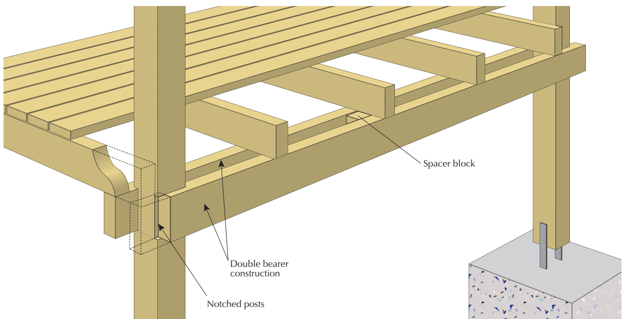
Figure 2: Notched posts with double bearers and spacer block construction
