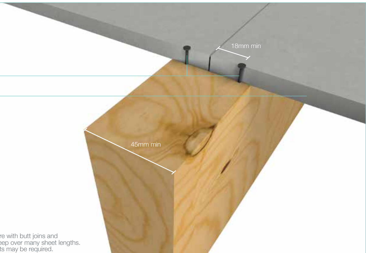
Figure 9 Butt Join
