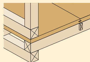
Platform construction
