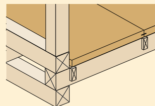
Fitted construction
