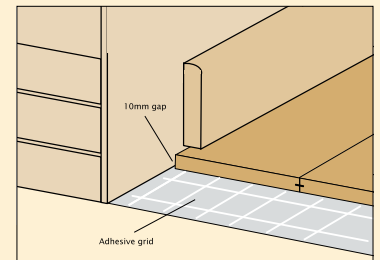
Particleboard flooring on Concrete Adhesive Bonded
