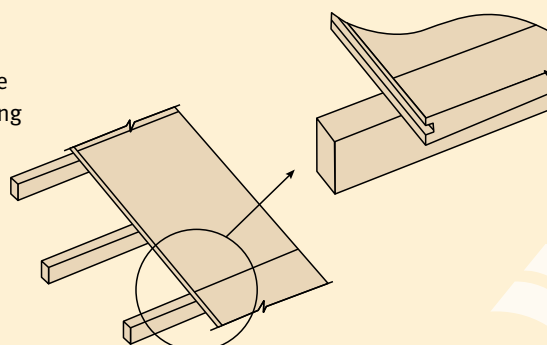
Platform construction
