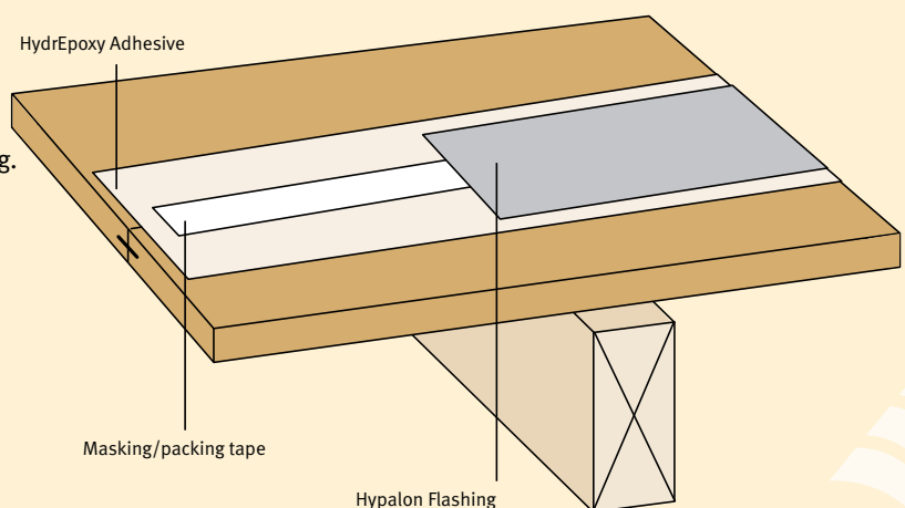
Sheet Join Flashing
