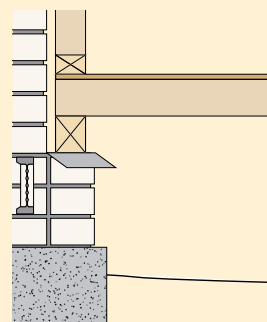
Platform construction
