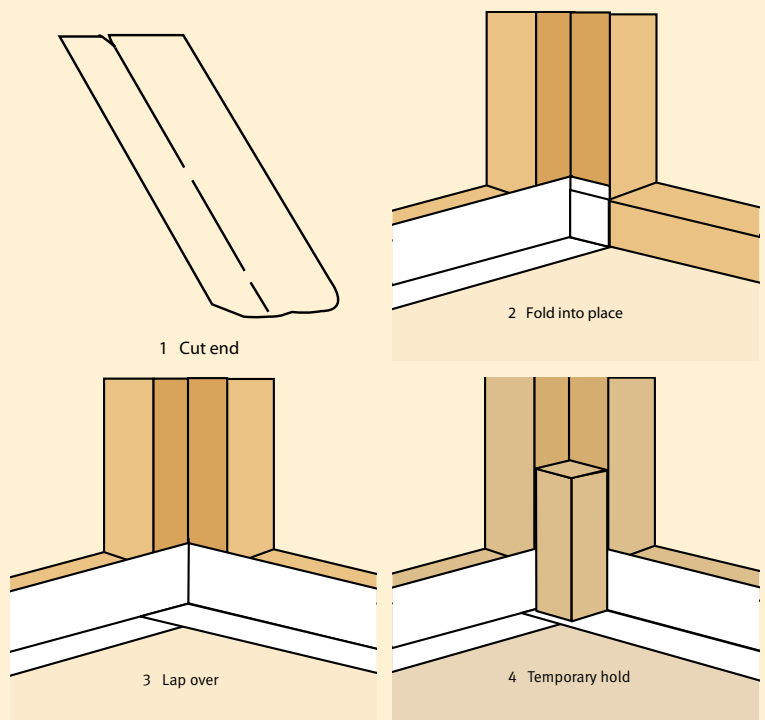
Vertical Flashing
