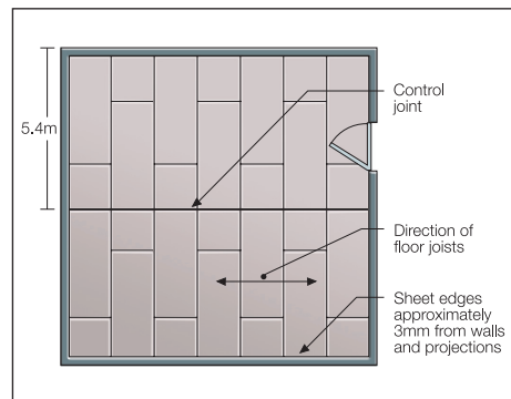
FIGURE 12 CONTROL JOINT LAYOUT
