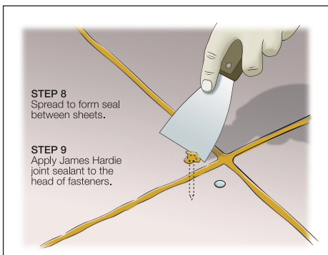
FIGURE 10 SEALING OVER FASTENERS - WET AREAS
