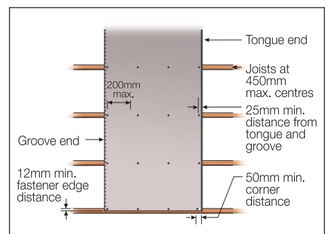
FIGURE 3 FASTENER LAYOUT
