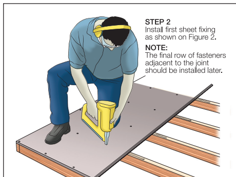
FIGURE 5 FIXING 1ST PANEL
