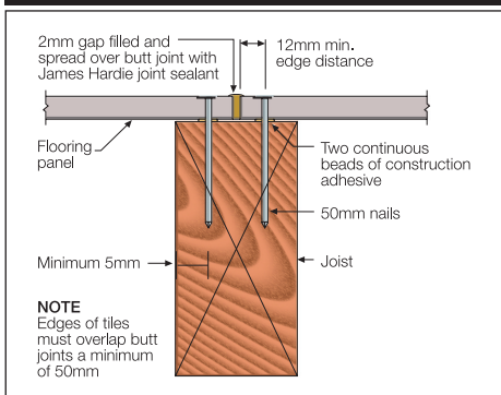
FIGURE 8 BUTT JOINT INTERNAL WET AREAS - TILE
