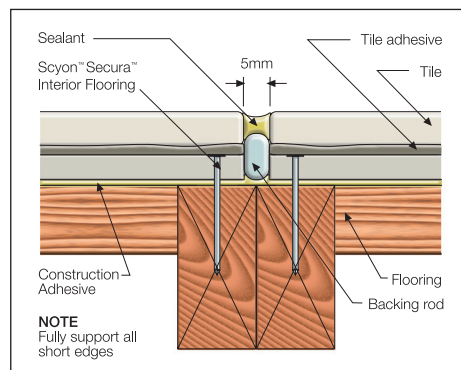
FIGURE 14 CONTROL JOINTS
