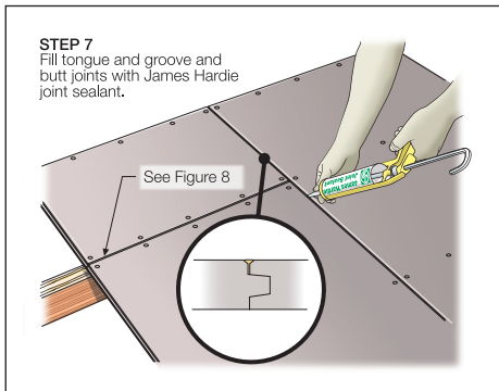
FIGURE 9 SEALING THE JOINTS IN WET AREAS - TILE
