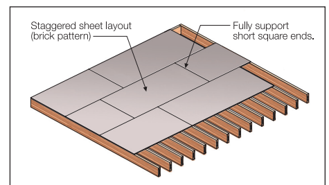
FIGURE 2 SHEET LAYOUT - TILING AND VINYL
