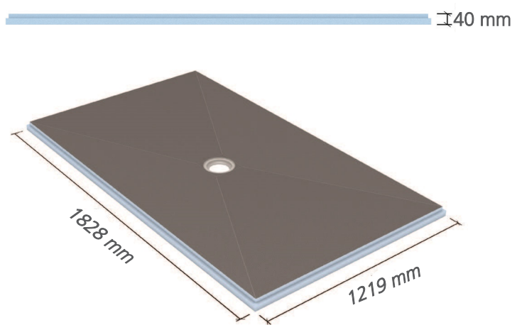
wedi Fundo Primo, rectangular 1219mm x 1828mm x 40mm 073742107
